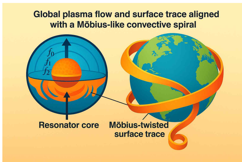
Figure 6. Conceptual illustration of the proposed resonant plasma model.
