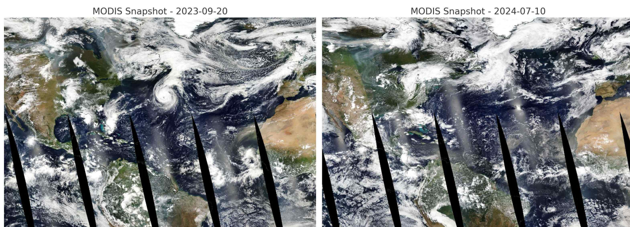
Figure 4. Satellite imagery shows increased atmospheric brightness linked to plasma activity. (Source: NASA Worldview, accessed July 10, 2024)
