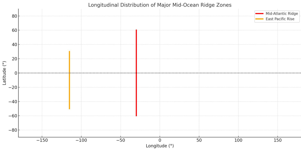
Figure 2. Asymmetry of global ridge zones suggests non-convective crustal dynamics. (Source: GEBCO Compilation Group, NOAA NGDC, accessed July 2024)
